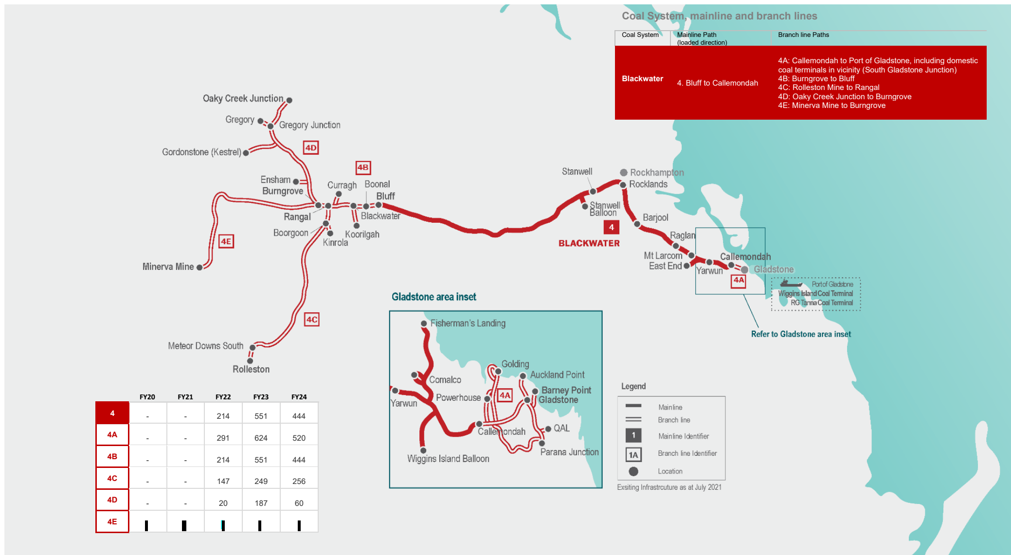
Figure 36 Blackwater Coal System ECDs (Train Paths)
